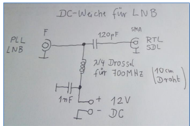
Circuit diagram of the bias tee
