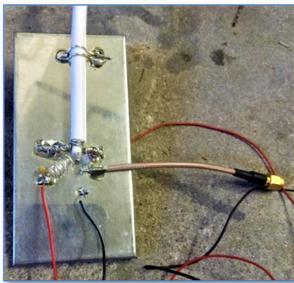
Quick and dirty build: The homemade bias tee
