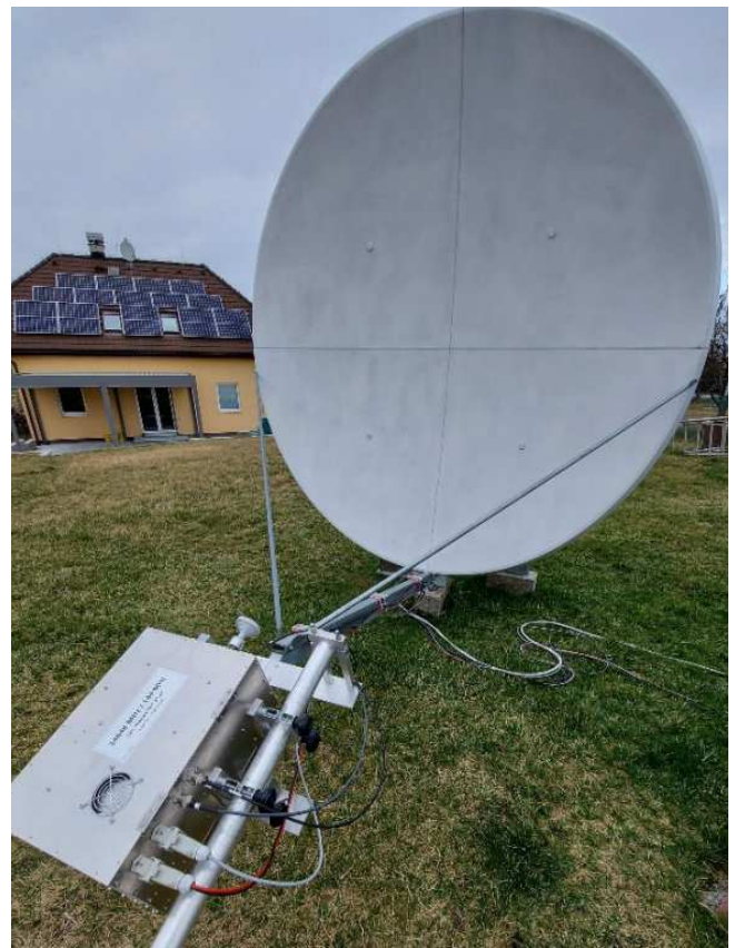
OK1DFC's 24 GHz setup
