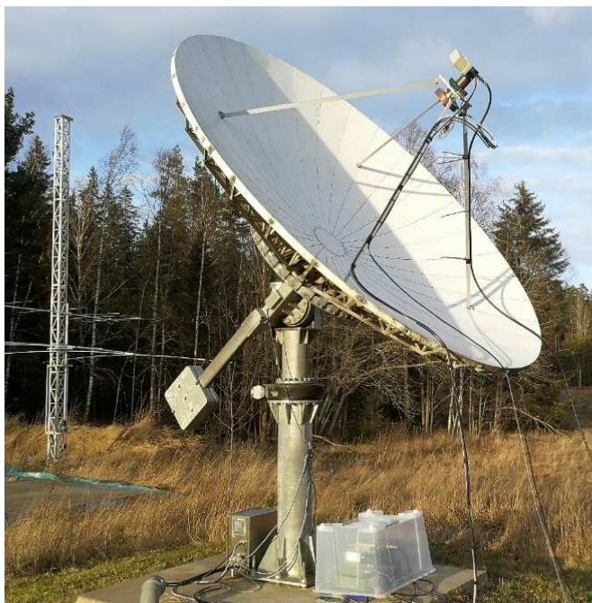
SA6BUN's 3 m dish and 9 cm equipment
