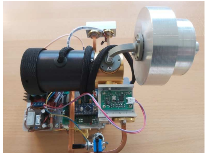
DL7YC 47GHz EME station (without SSPA)
