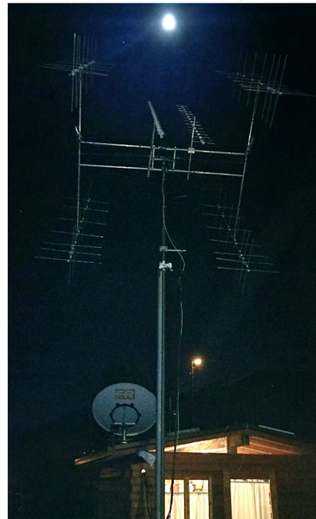
IW2FZR's EME antennas at home QTH with 1.8 m dish
